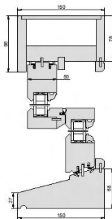
Sash Weights WPL SBD 150
