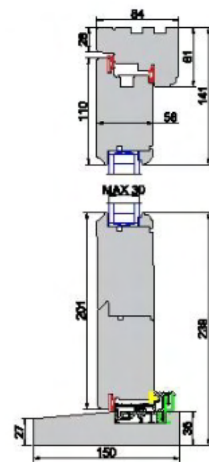
French Door 58 opening outside
