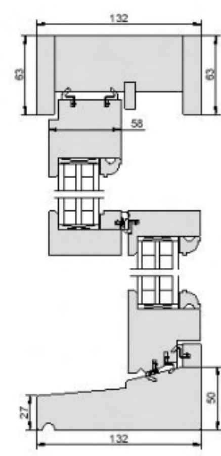
Sash Tilt & Slide 58/63
