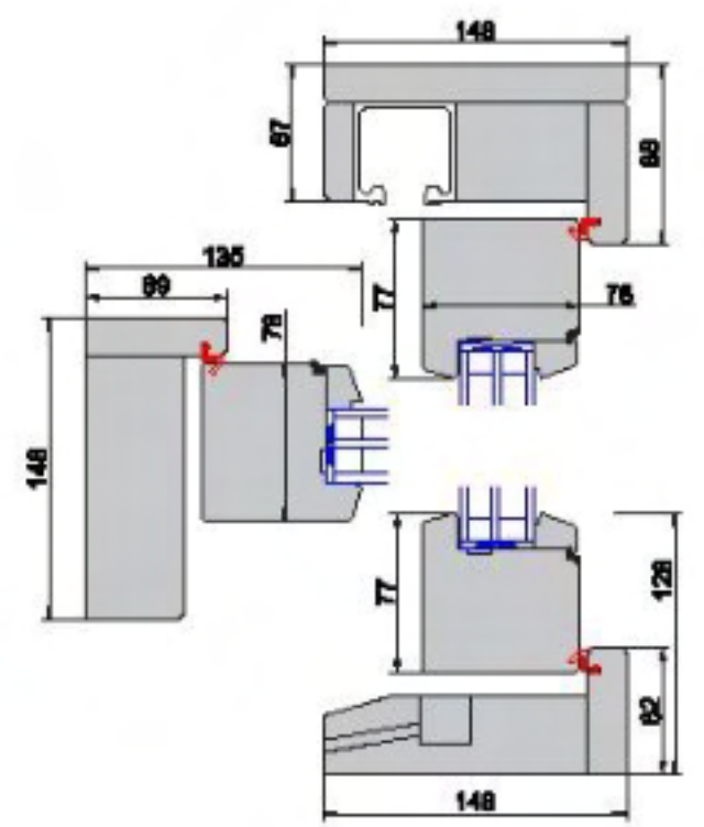
Bi-Folding 78
