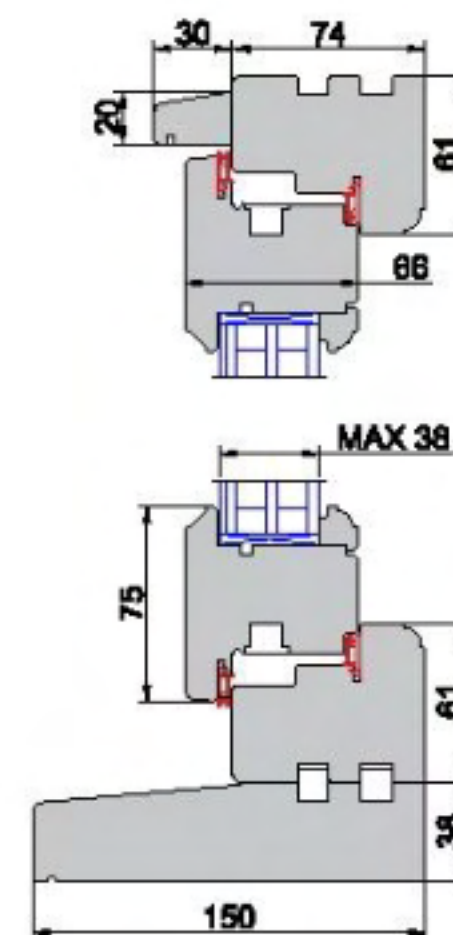
Stormproof 66/74 drip + cill 150/38
