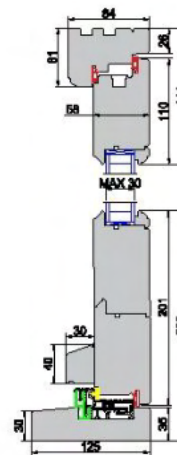
French Door 58 opening inside
