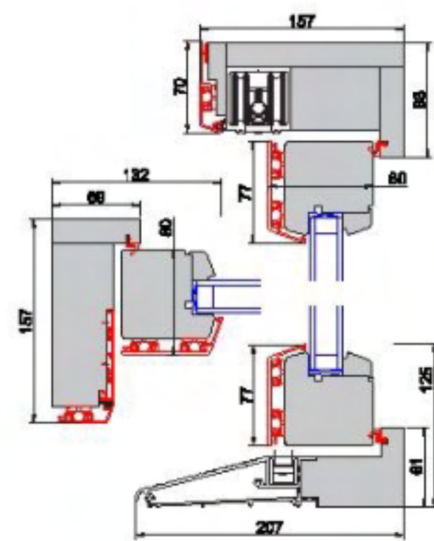
Bi-Folding Aluclad
