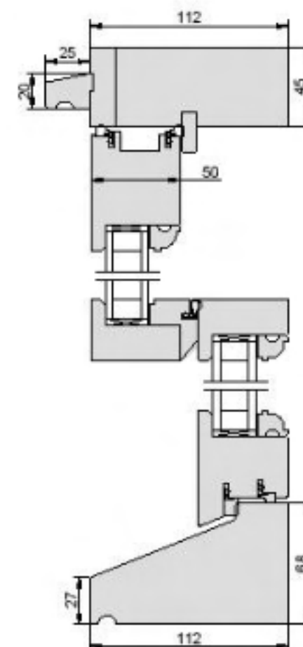
Mock Sash Traditional Flush 50/45
