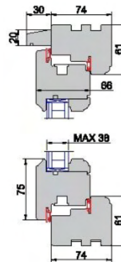
Stormproof 66/74 drip
