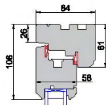
Flush 58/84
