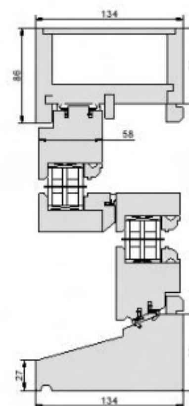
Sash Weights Excellent 58/86
