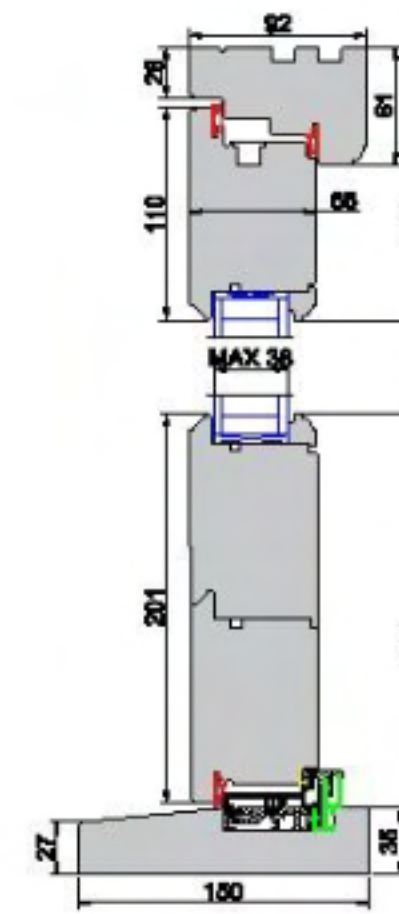
French Door 66 opening outside
