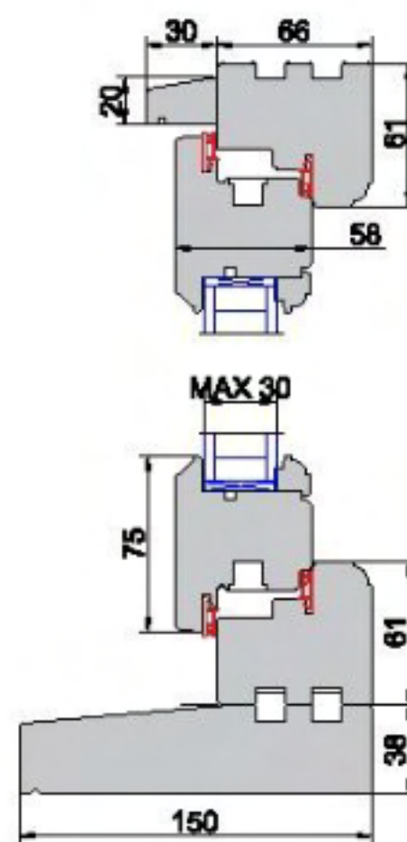
Stormproof 58/66 drip + cill 150/38
