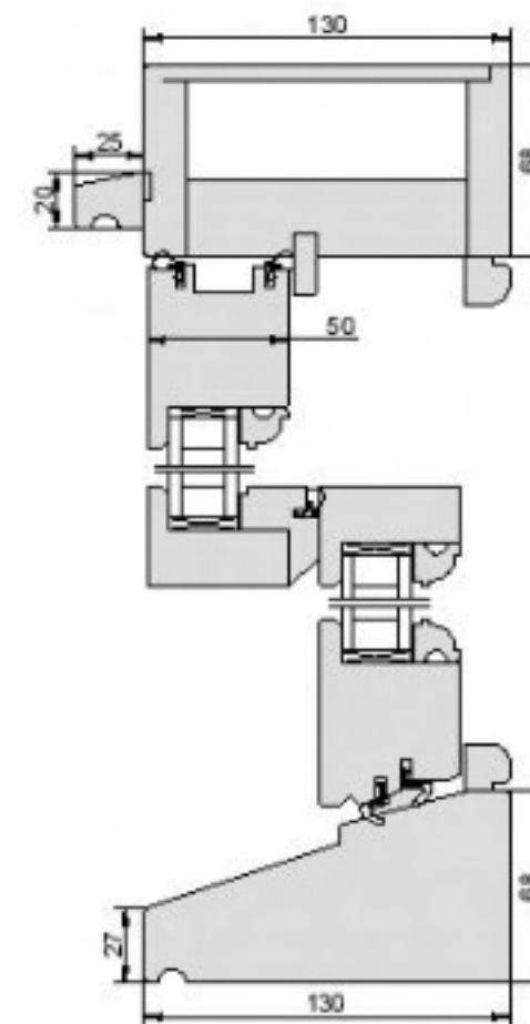
Mock Sash Tilt & Slide 50/68
