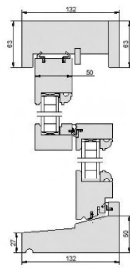
Sash Tilt & Slide 50/63
