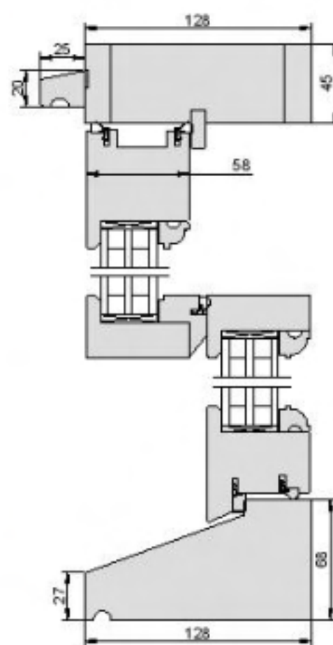
Mock Sash Traditional Flush 58/45
