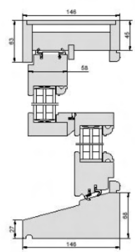
Sash Balance Elegance 58/63
