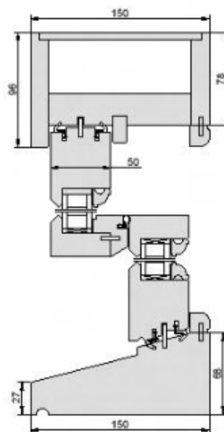
Sash Balance BPL SBD 150
