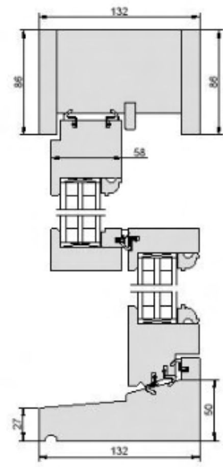
Sash Tilt & Slide 58/86
