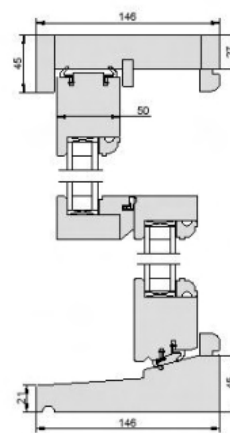
Sash Balance 50/45
